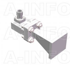
LB-28-15-64-C-KFSPO Frequency Extended Standard Gain Horn Antenna 22.5-45GHz 15dB Gain 2.92mm Female
